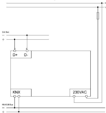
Exemplary circuit diagram SCN-DALI64.02
